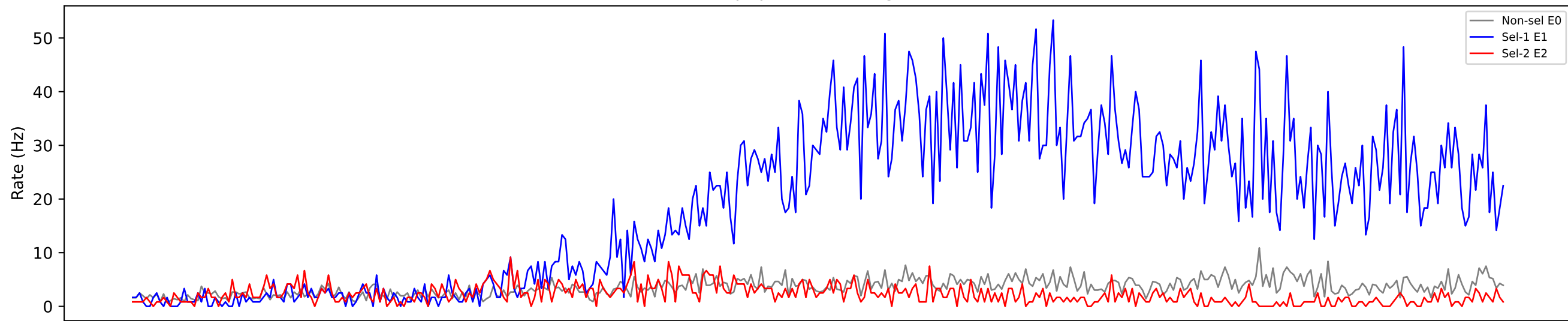
E Subpopulation Firing Rates
